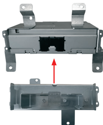
Slide the screen support onto the the radio unit
