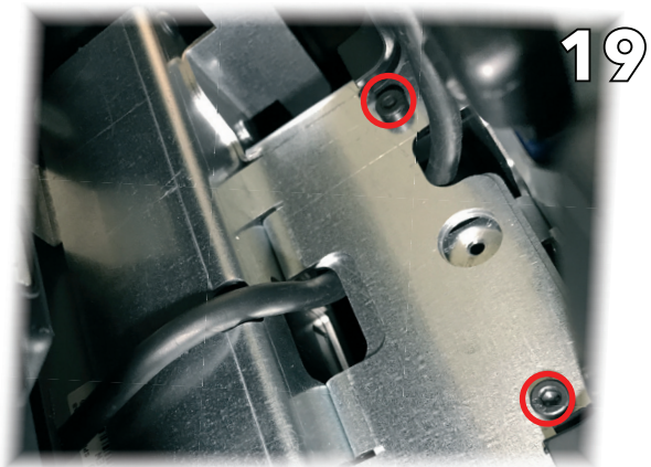
Secure the display in its position using the 2 indicated screw points
