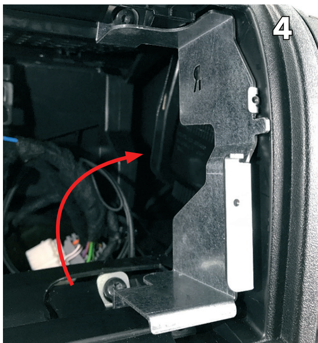
Install right side bracket using the van's original torx screw
