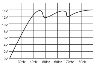
Bassperformanze at 50Hz and 70Hz without capacitor
