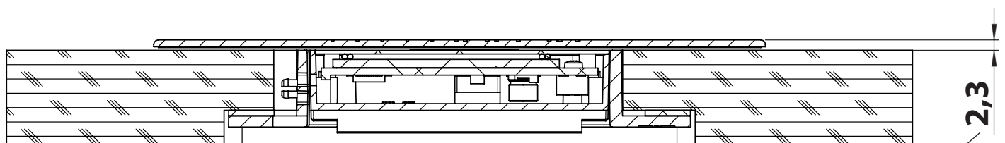
Abstand-Filterborad zur Anwendungsfläche: 2,3 mm Distance surface filter-board to application surface: 2,3 mm
