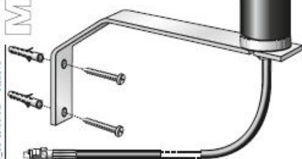
Stations-Antenne mit Stabstrahler Antenna for Basic Station with radiation rod
